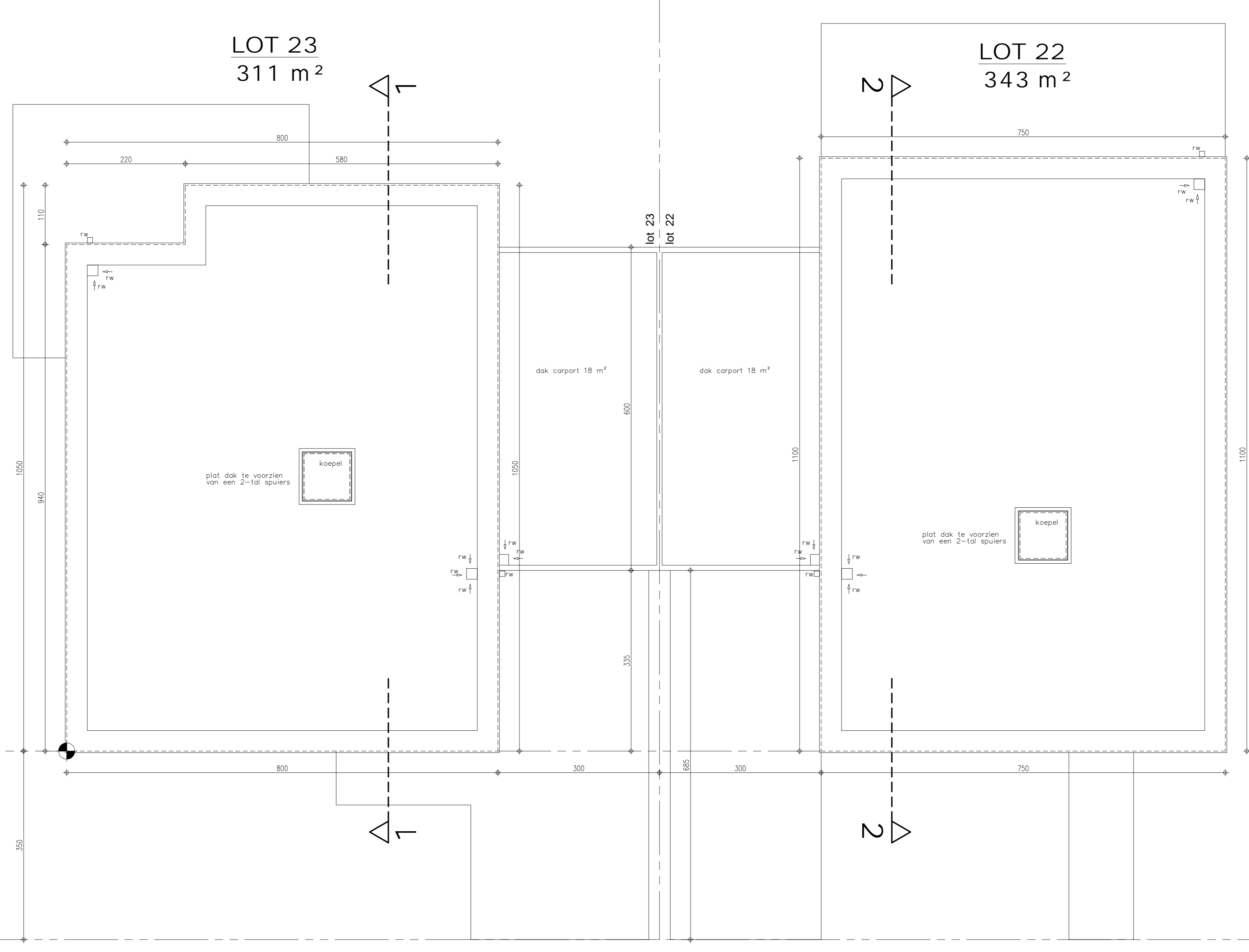
DAKENPLAN 1/50
